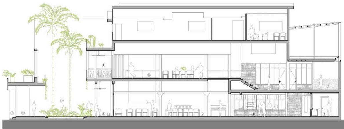
TRANSVERSAL SECTION
